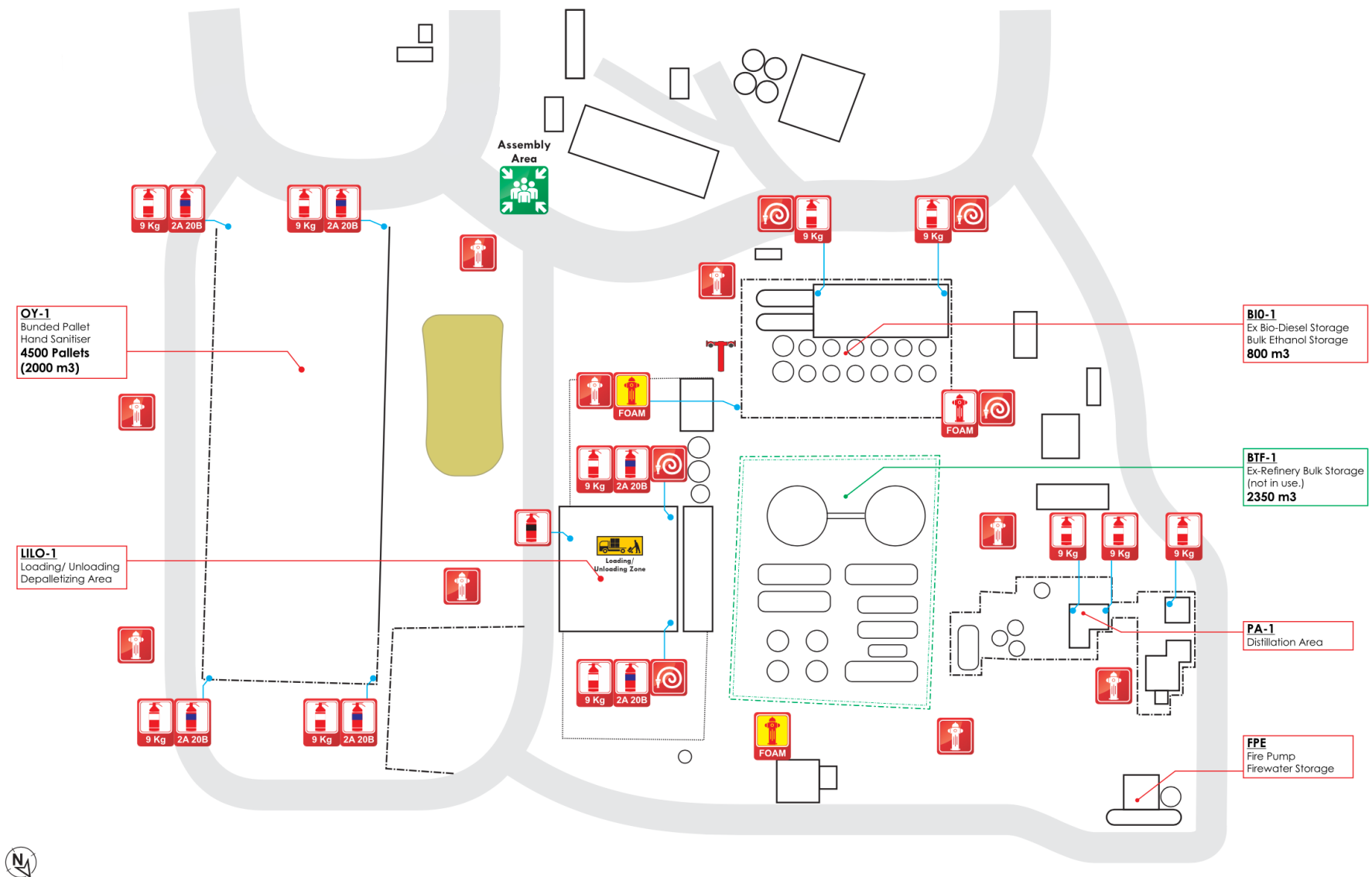
Figure 1. Floor Plan
